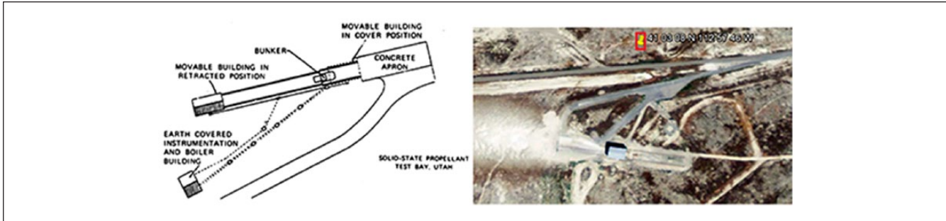
Figure 3. Schematic drawing of test facility and a current Google Earth photo of the site. Note. The box in the upper portion of the photo represents the location of the geographical coordinates.
